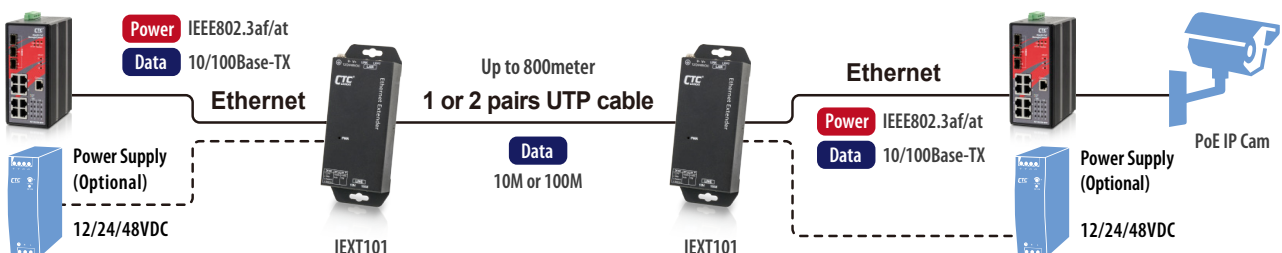
Figure2 : Long distance data transmission application
