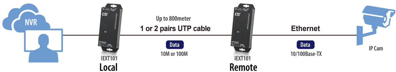
Figure1 : Long distance data transmission application
