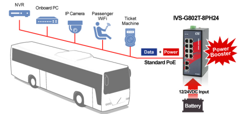
E-Mark certified PoE switch for in-vehicle network applications
